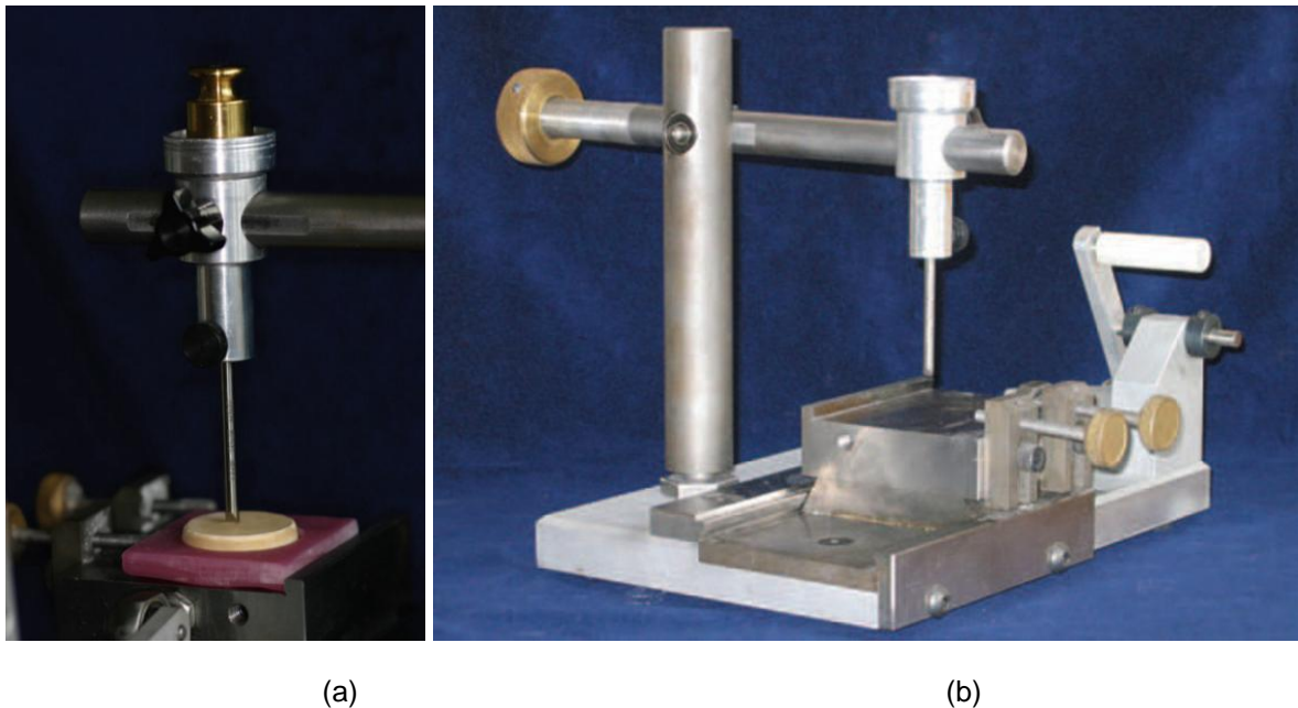
Fig. 3. Two body wear test apparatus
