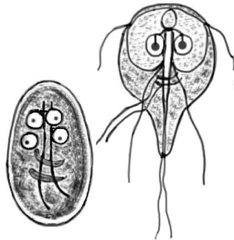
Fig. 3. Giardia lamblia Cyst (Left) and Trophozoite (Right) (Source: CDC, 2007)
