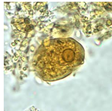
Fig. 4. Entamoeba histolytica Trophozoite in a Direct Wet Mount Stained with Iodine (Source: CDC, 2019)
