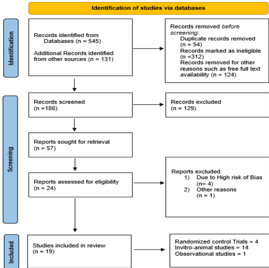
Fig. 1. PRISMA 2020 flow diagram for systematic reviews, which included searches of databases, registers and other sources
