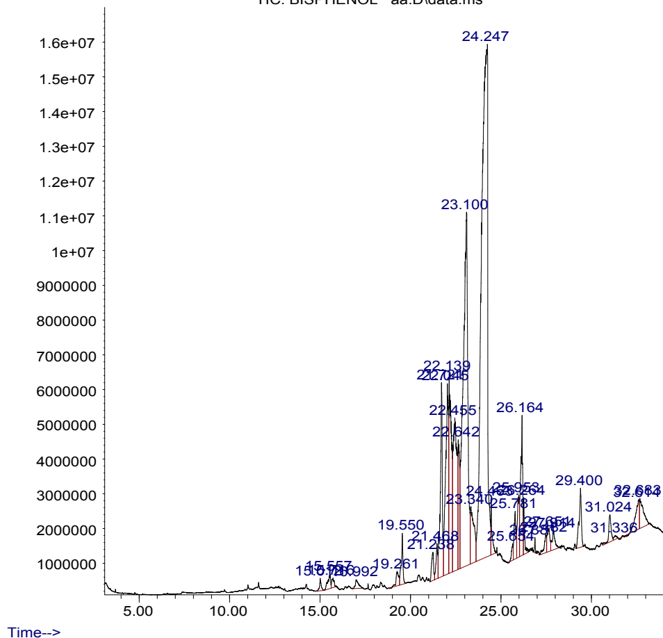
Fig. 5. Gas Chromatography/Mass Spectrometry chromatogram of Tomato paste extract. Retention Time: BPA-15.0 min.
