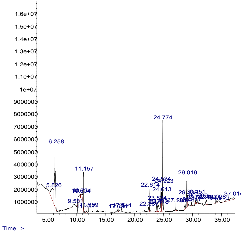
Fig. 3. Gas Chromatography/Mass Spectrometry chromatogram of sweet corn extract.
