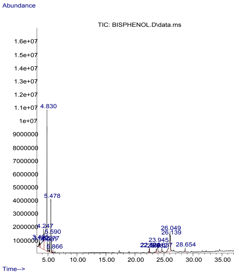
Fig. 4. Gas Chromatography/Mass Spectrometry chromatogram of Sardine Extract. Retention Time: No presence of BPA
