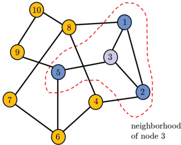
Figure 1. Graphical representation of a network with 10 nodes. Edges represent which nodes can communicate. The red area depicts the node’s neighborhood \mathcal{N}_3 \subseteq \mathcal{V}, \mathcal{N}_3 = \{1, 2, 3, 5\} .
